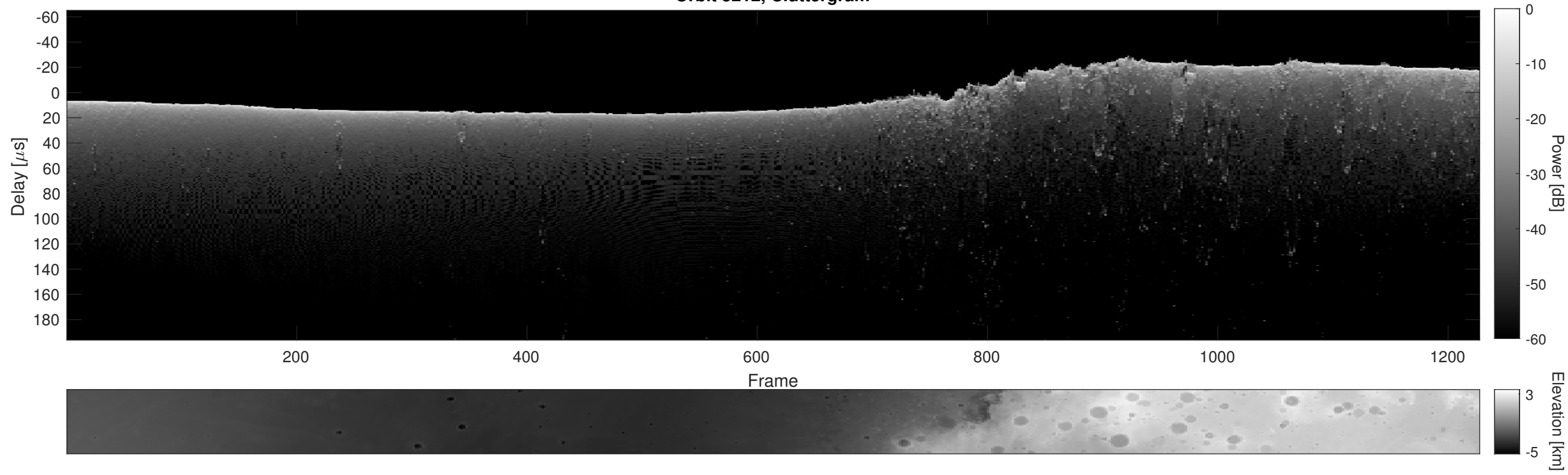
Orbit 5212, Cluttergram
