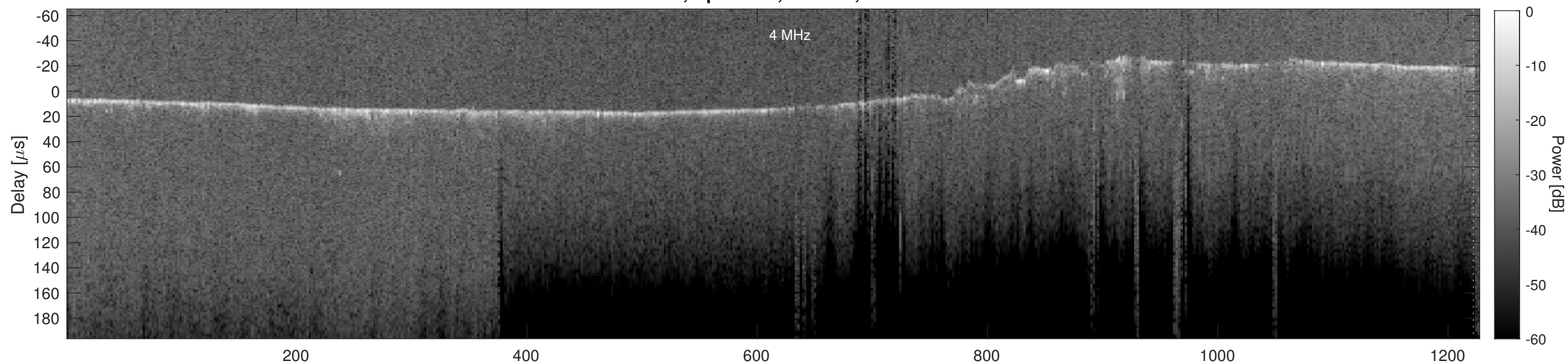
Orbit 5212, Cluttergram
