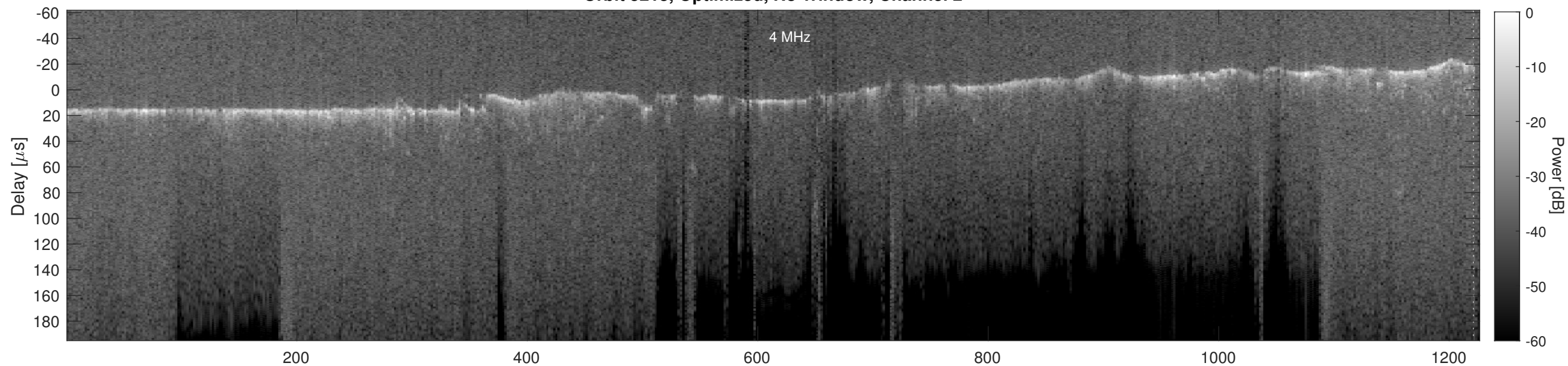
Orbit 5213, Cluttergram
