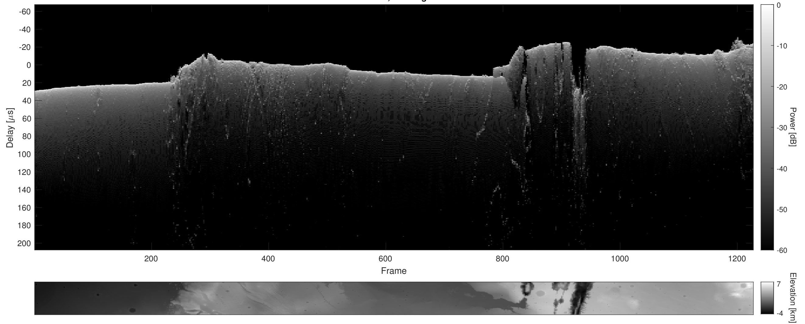
Orbit 5214, Cluttergram
