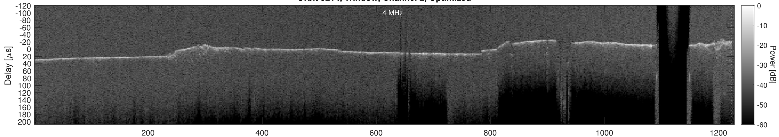
Orbit 5214, Cluttergram
