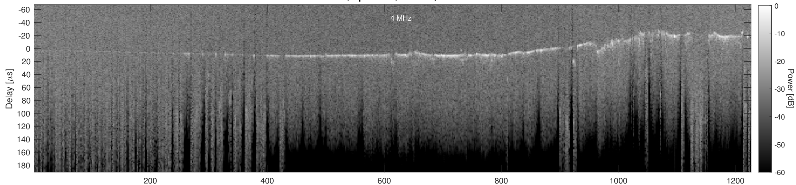
Orbit 5215, Cluttergram
