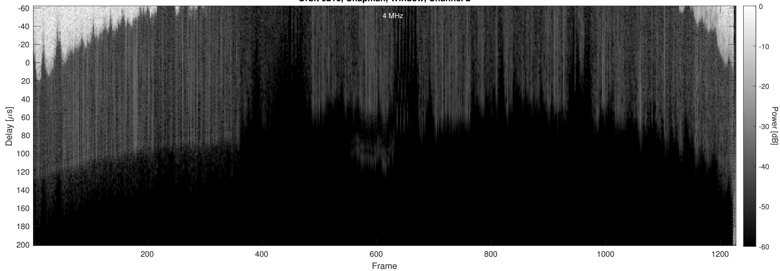
Orbit 5216, Chapman, Window, Channel 2
