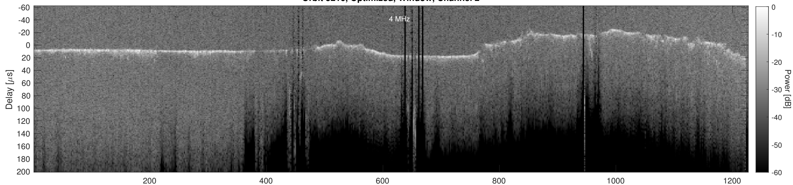
Orbit 5216, Cluttergram
