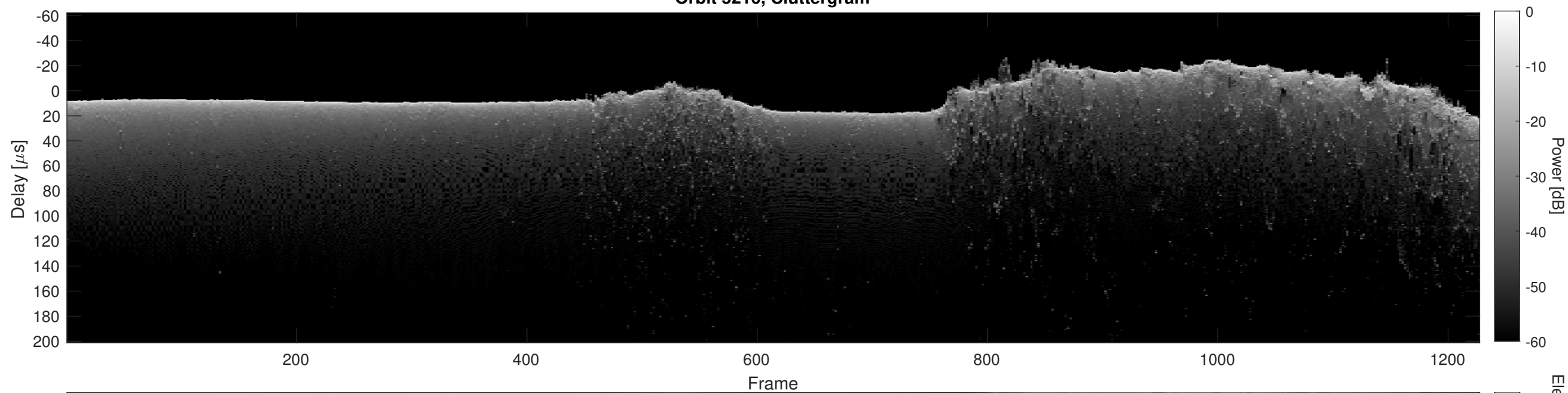
Orbit 5216, Cluttergram
