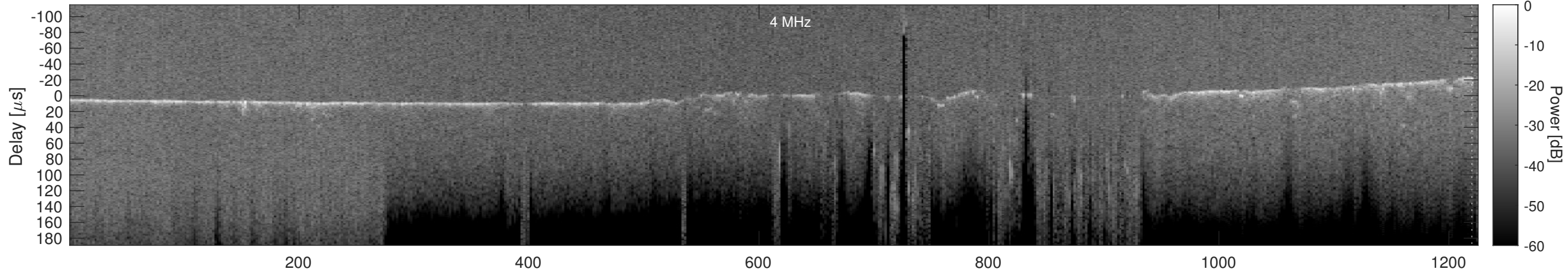
Orbit 5217, Cluttergram
