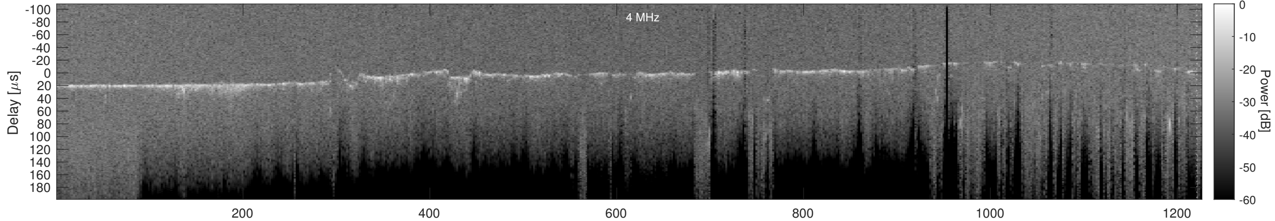
Orbit 5220, Cluttergram
