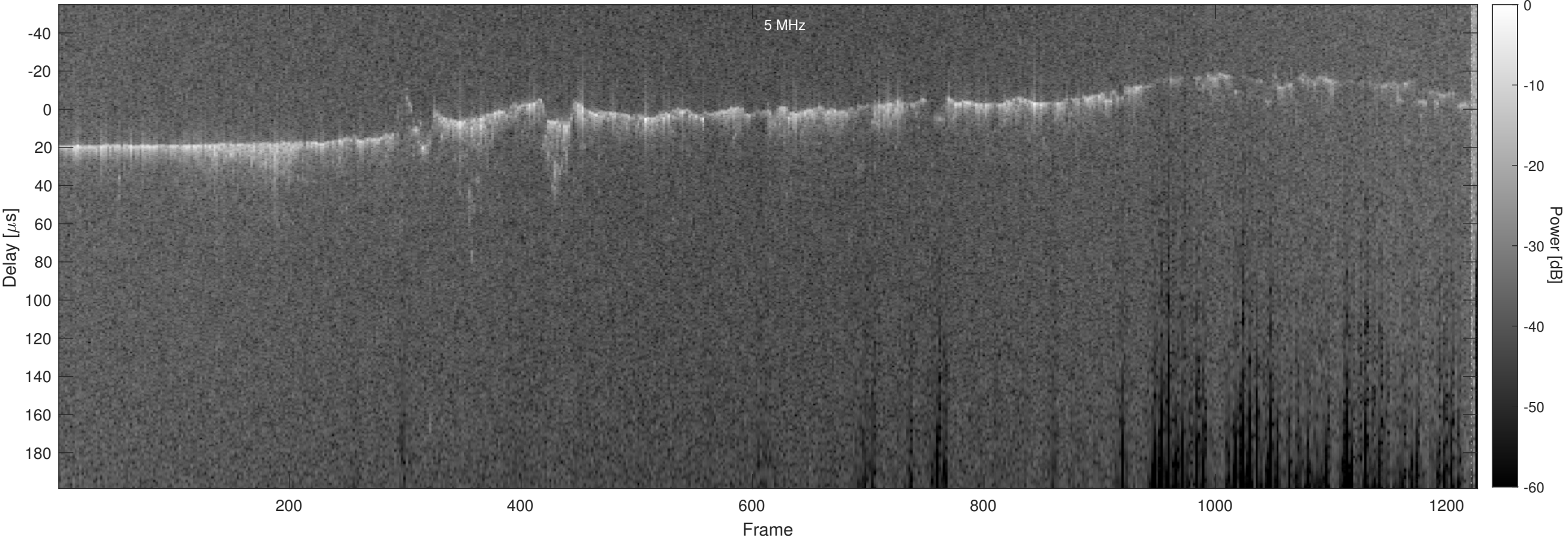
Orbit 5220, Optimized, No Window, Channel 2
