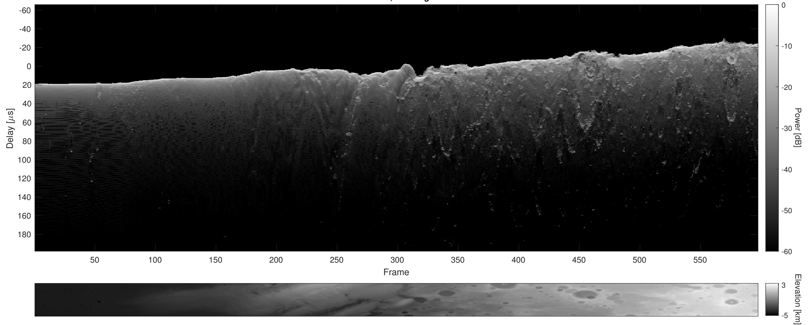
Orbit 5222, Cluttergram
