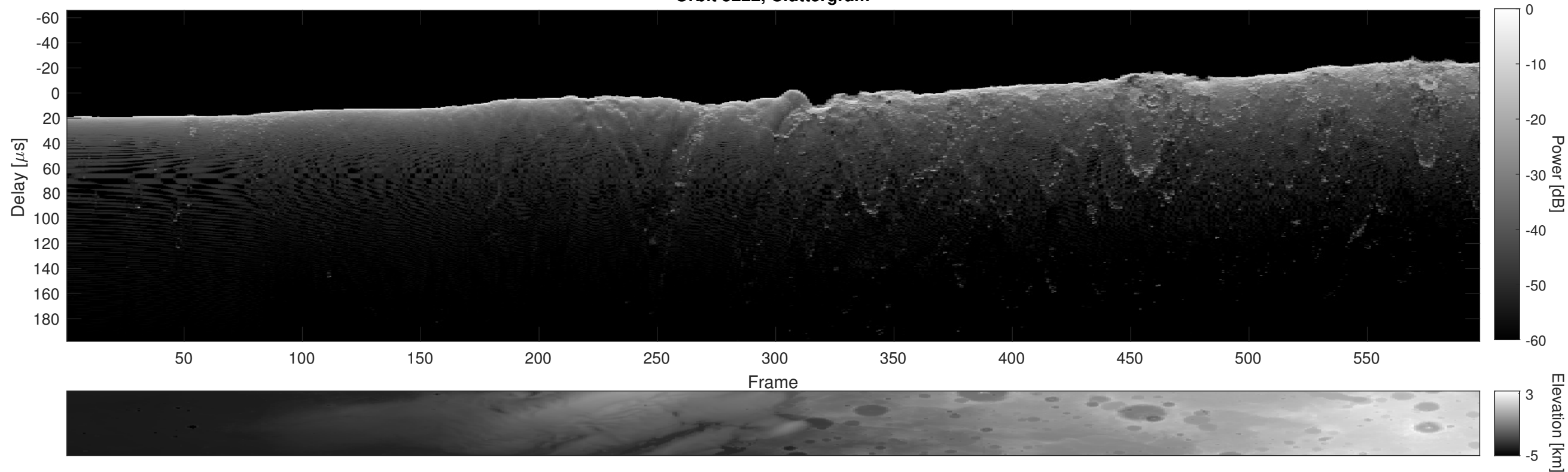
Orbit 5222, Cluttergram
