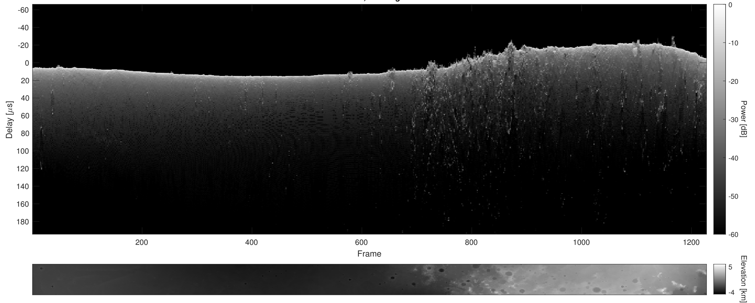
Orbit 5223, Cluttergram
