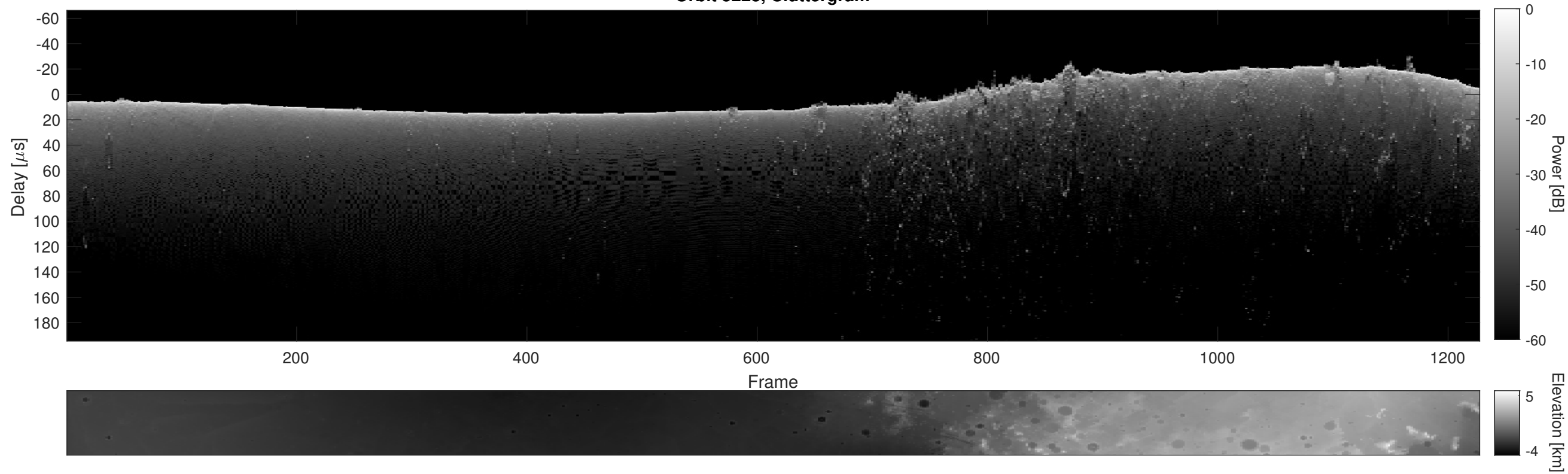
Orbit 5223, Cluttergram
