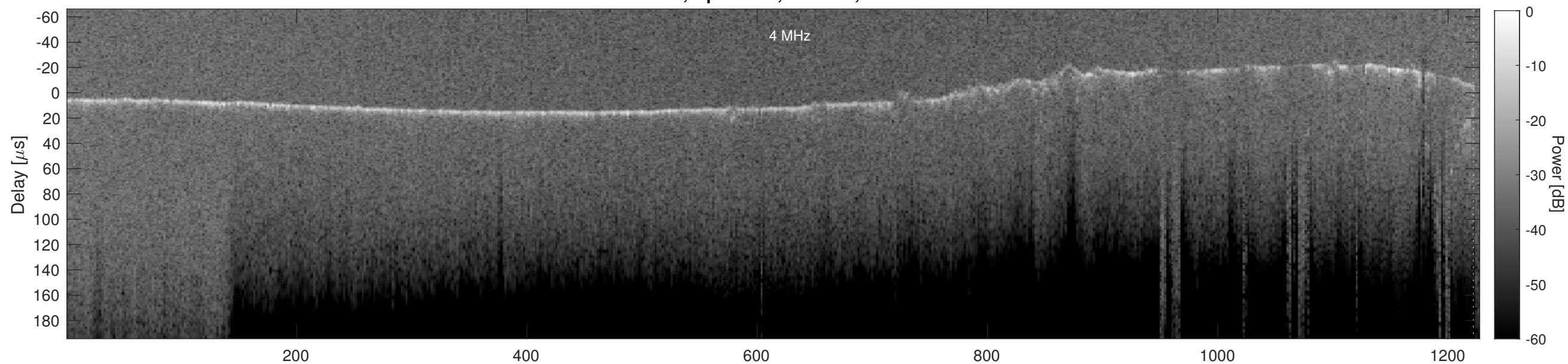
Orbit 5223, Cluttergram
