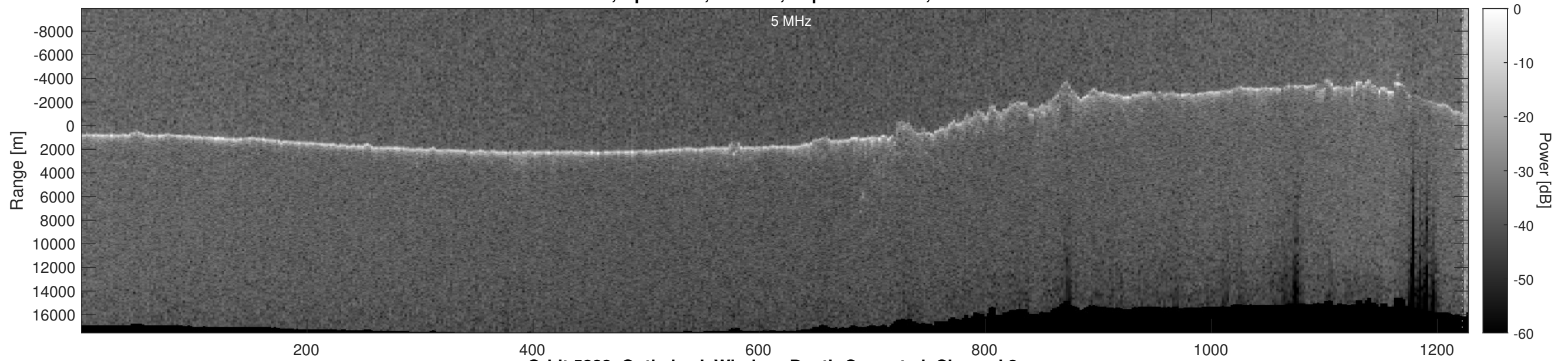
Orbit 5223, Optimized, Window, Depth-Corrected, Channel 2
