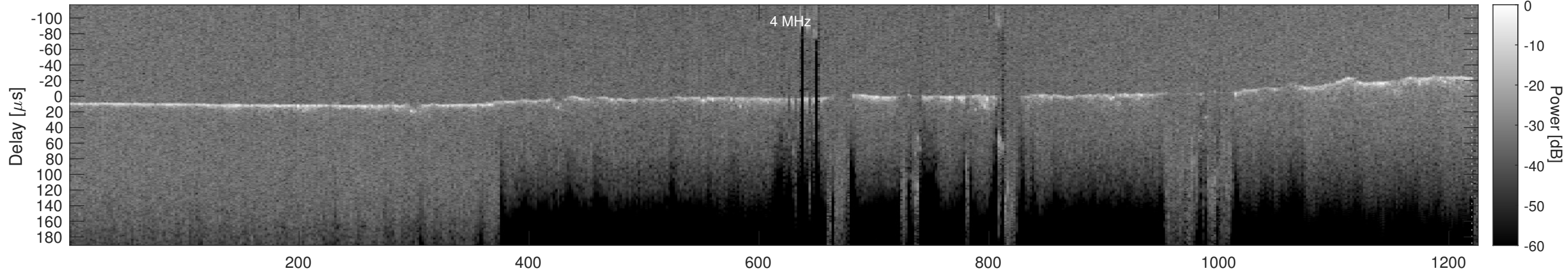
Orbit 5224, Cluttergram
