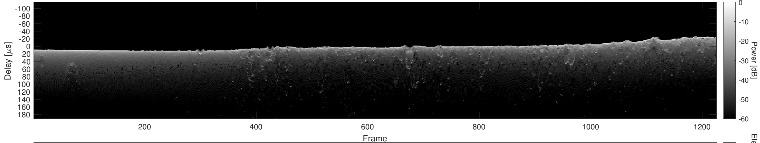
Orbit 5224, Cluttergram
