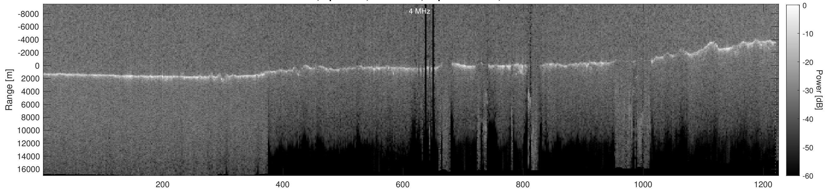
Orbit 5224, Depth-Corrected Cluttergram
