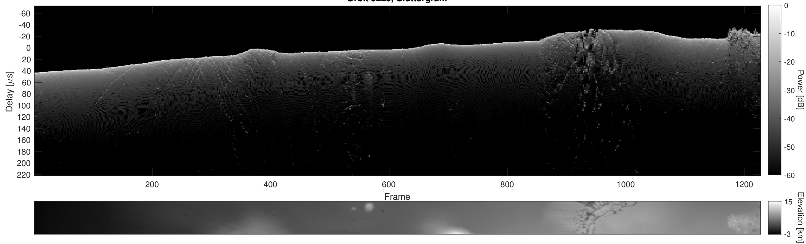
Orbit 5225, Cluttergram
