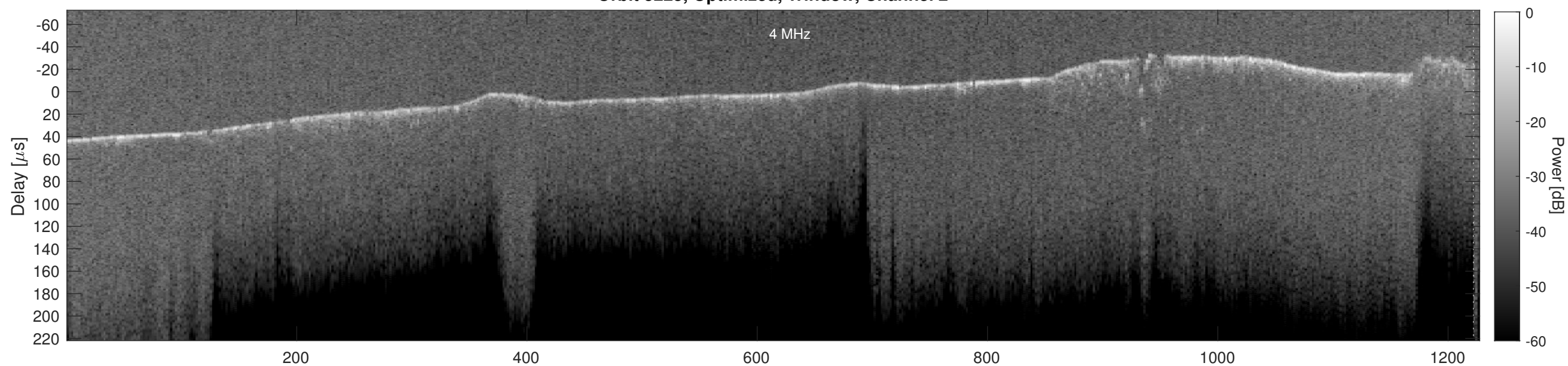
Orbit 5225, Cluttergram
