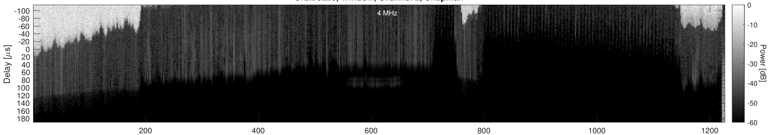
Orbit 5226, Window, Channel 2, Optimized
