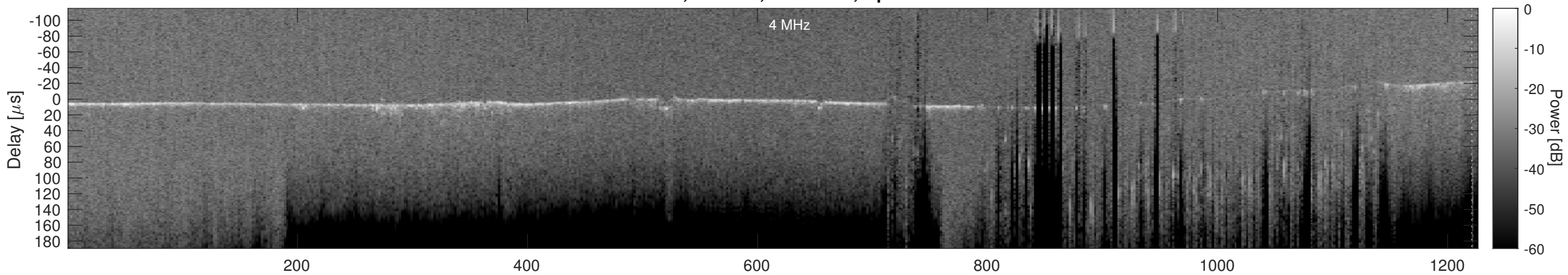
Orbit 5226, Cluttergram
