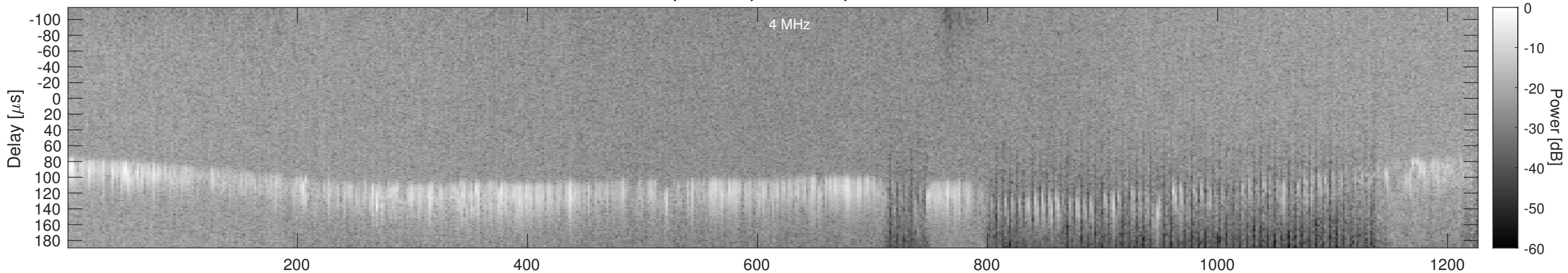
Orbit 5226, Window, Channel 2, Chapman
