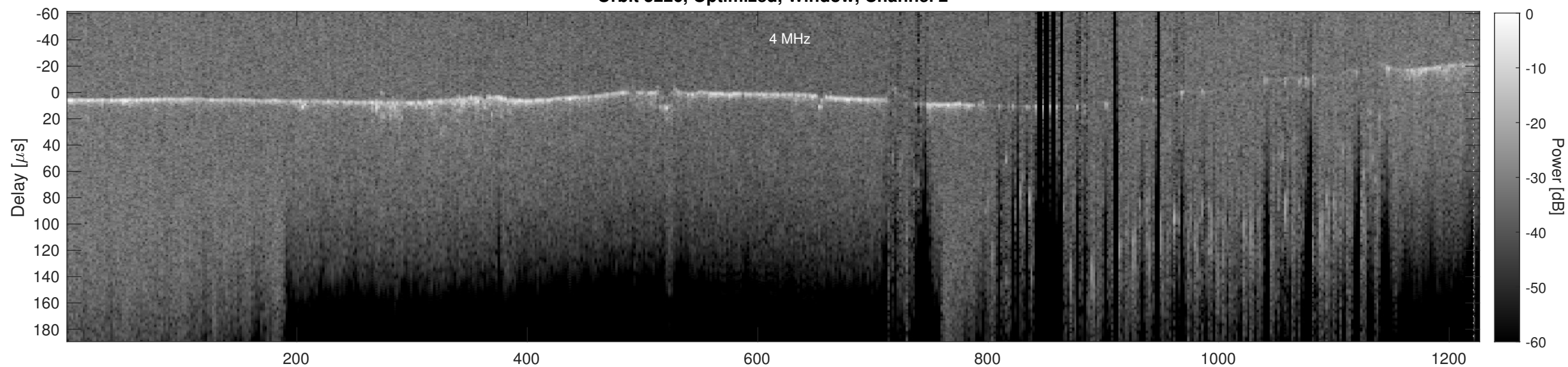
Orbit 5226, Cluttergram
