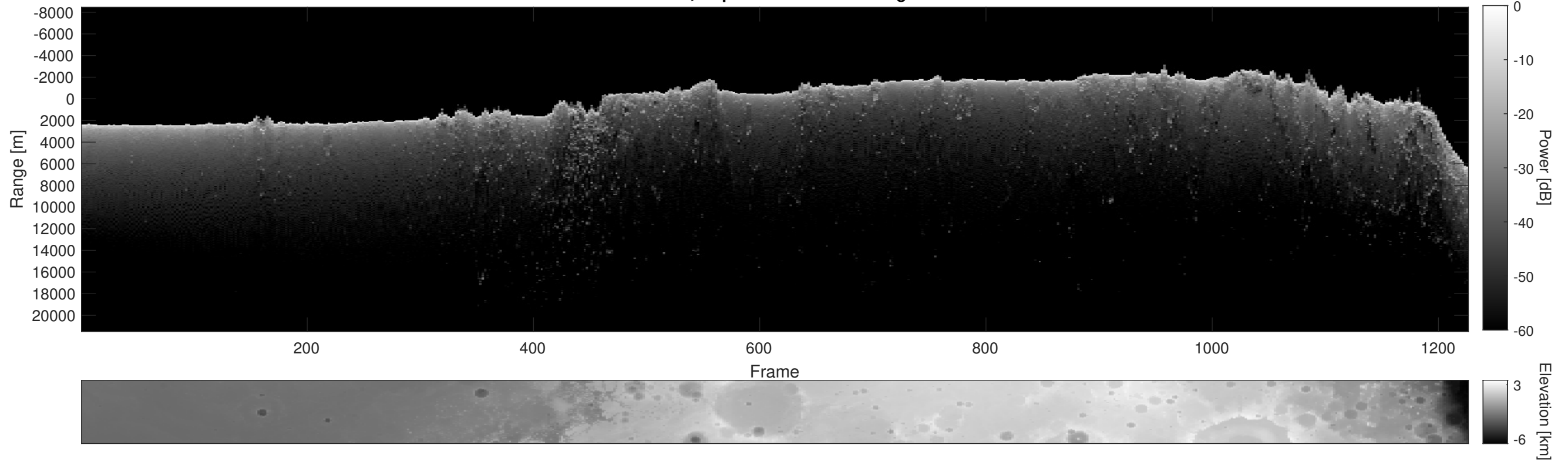
Orbit 5227, Depth-Corrected Cluttergram
