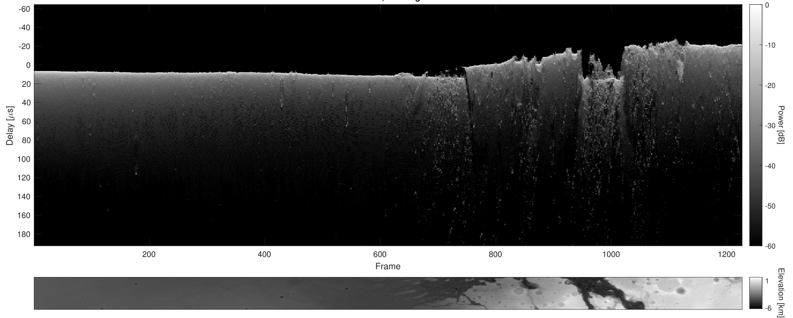
Orbit 5228, Cluttergram
