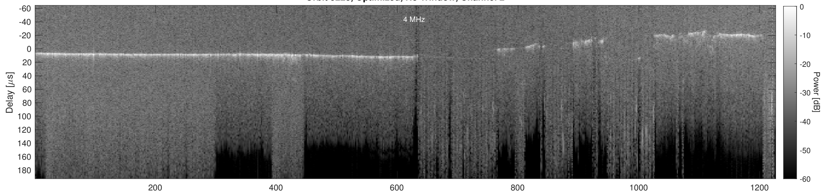
Orbit 5228, Cluttergram
