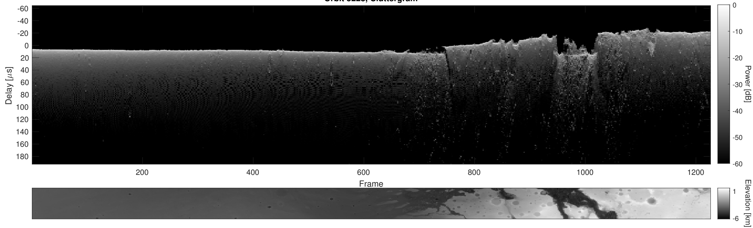
Orbit 5228, Cluttergram
