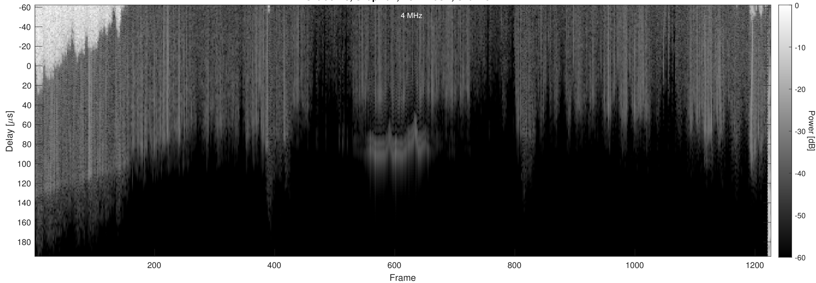
Orbit 5229, Chapman, No Window, Channel 2
