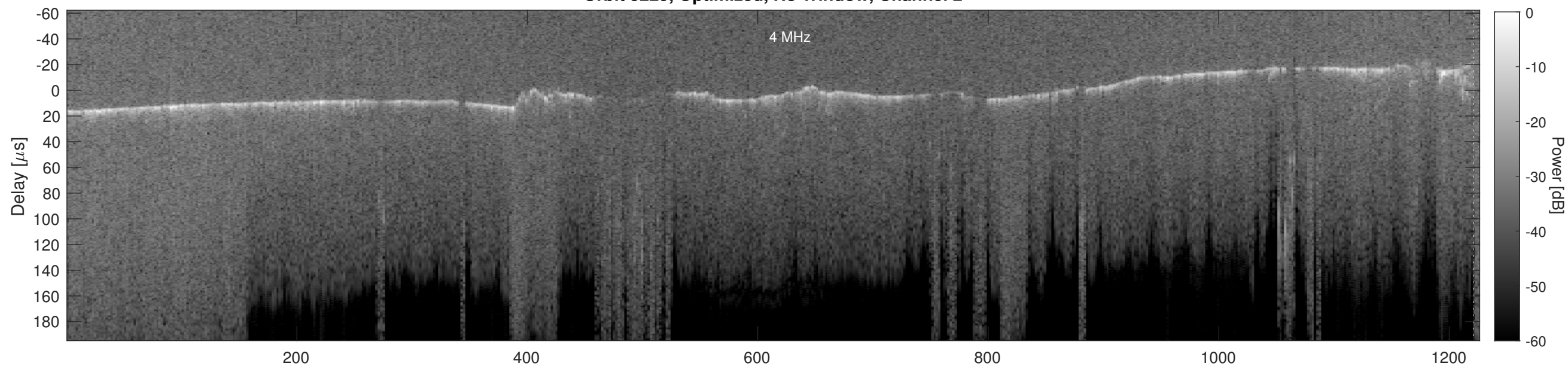
Orbit 5229, Cluttergram
