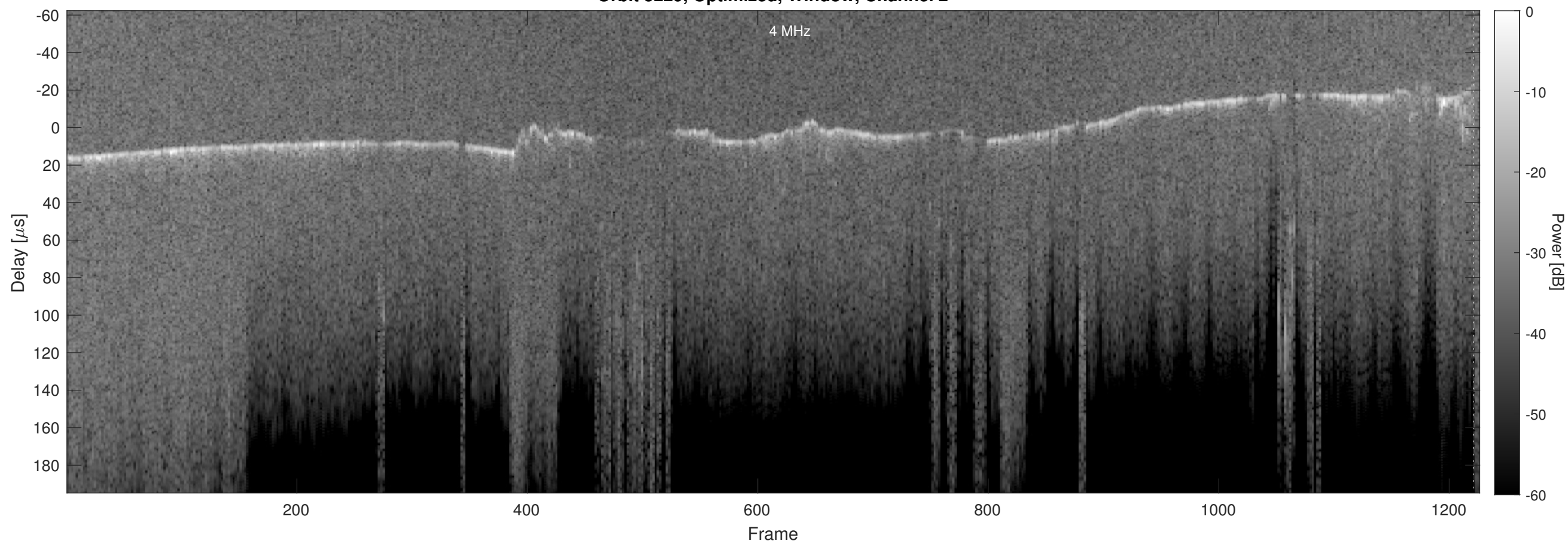
Orbit 5229, Optimized, Window, Channel 2
