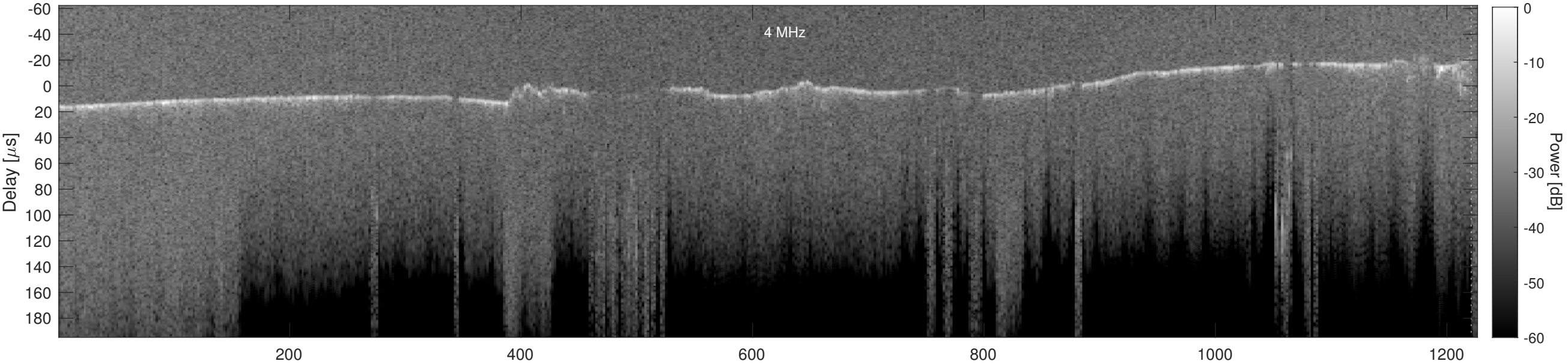
Orbit 5229, Cluttergram
