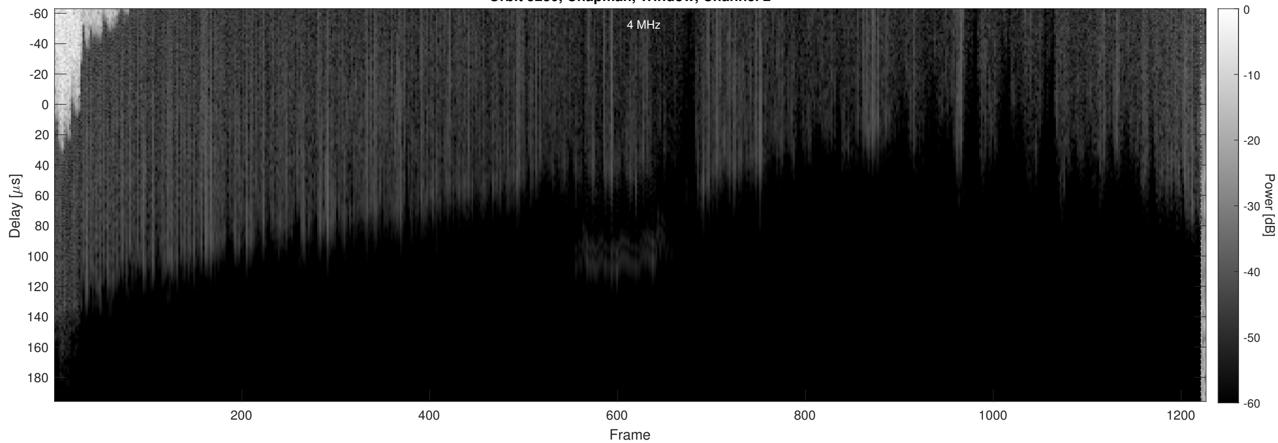
Orbit 5230, Chapman, Window, Channel 2
