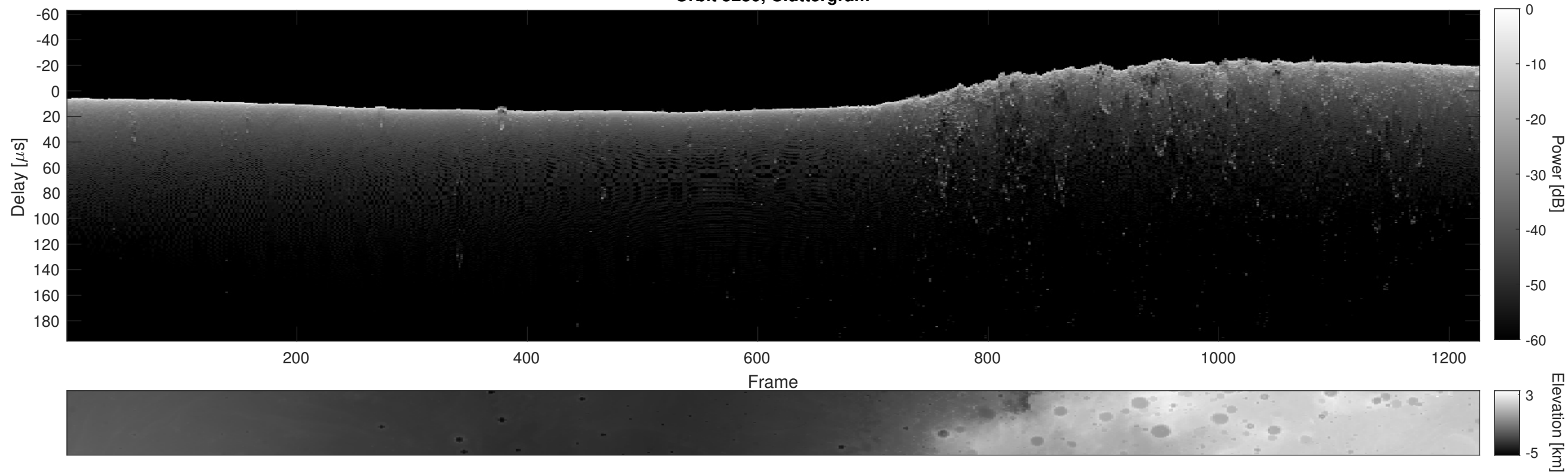
Orbit 5230, Cluttergram
