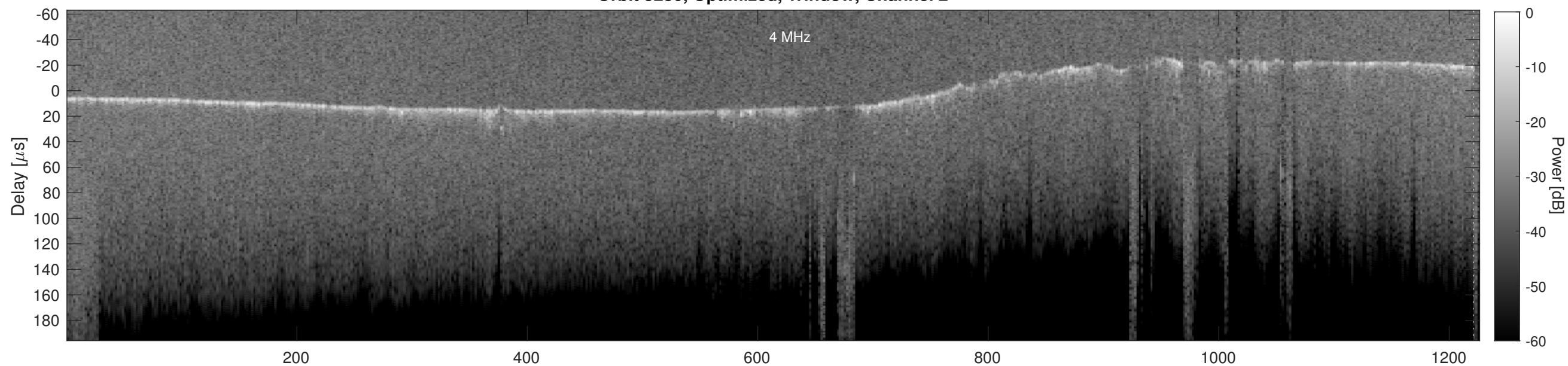
Orbit 5230, Cluttergram
