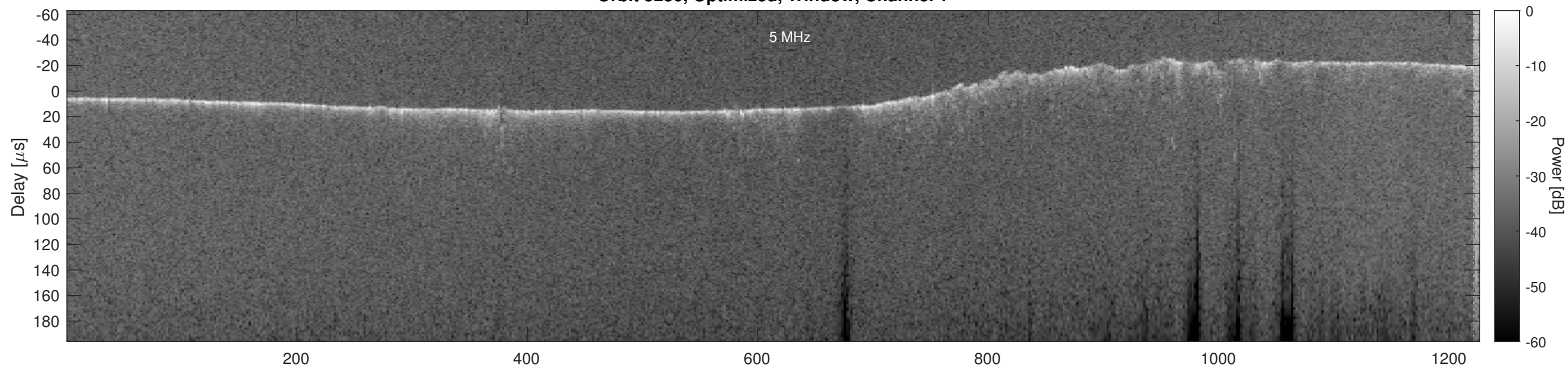
Orbit 5230, Optimized, Window, Channel 2
