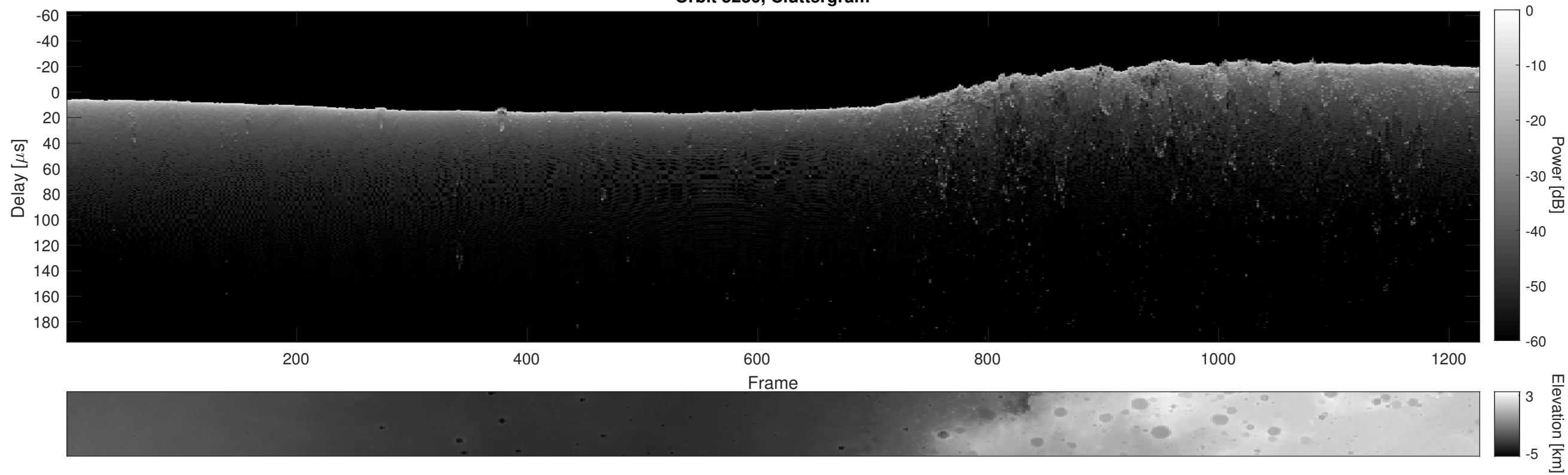
Orbit 5230, Cluttergram
