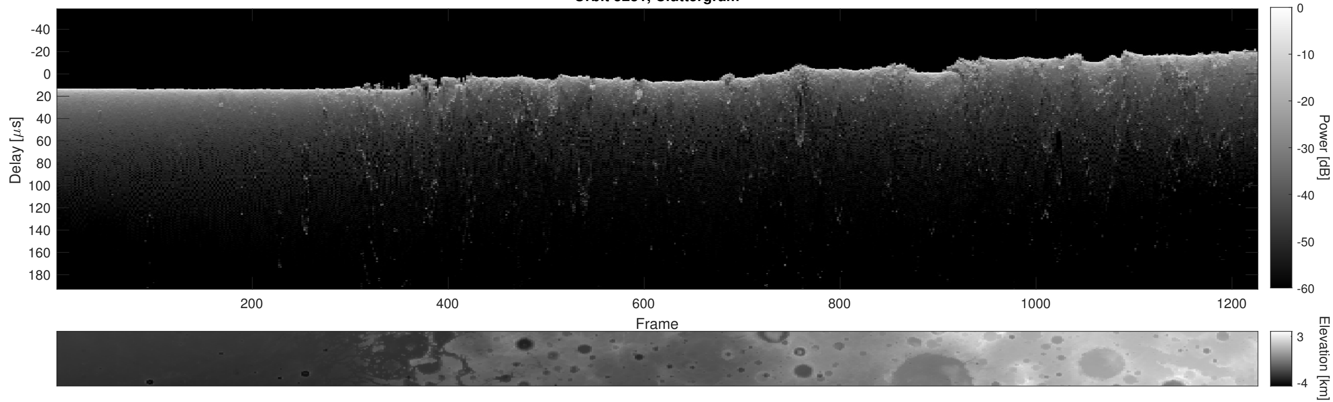
Orbit 5231, Cluttergram
