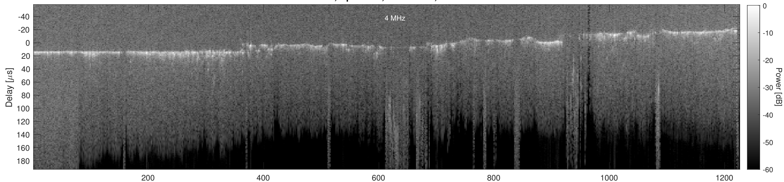
Orbit 5231, Cluttergram
