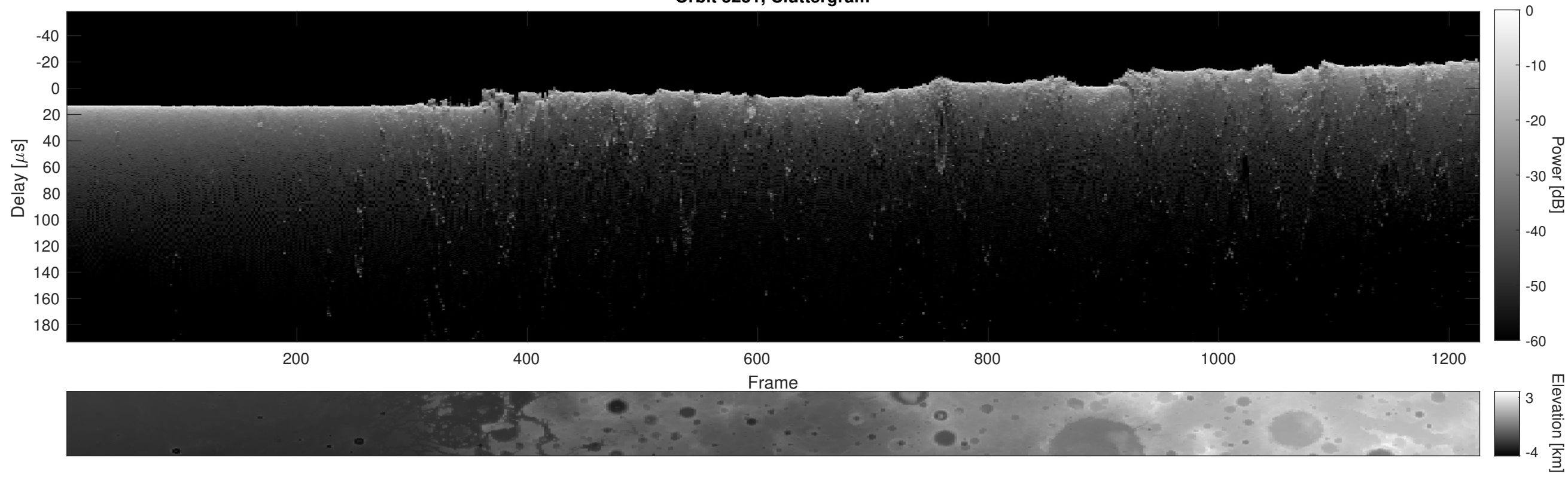
Orbit 5231, Cluttergram
