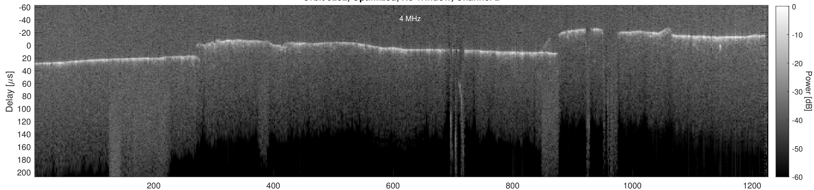
Orbit 5232, Cluttergram
