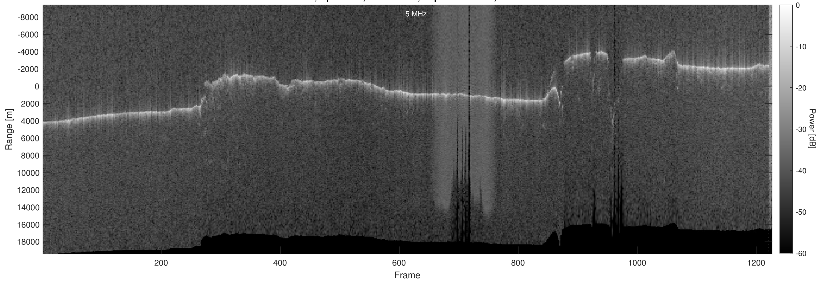
Orbit 5232, Optimized, No Window, Depth-Corrected, Channel 2
