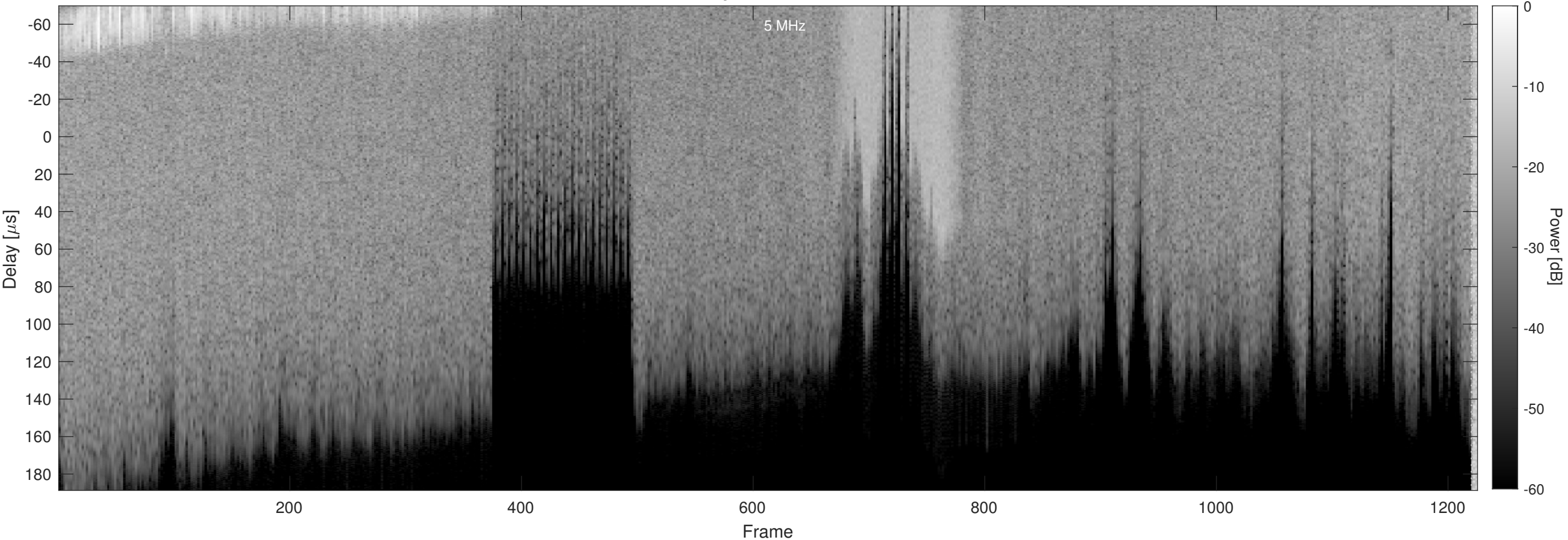
Orbit 5233, Chapman, Window, Channel 2
