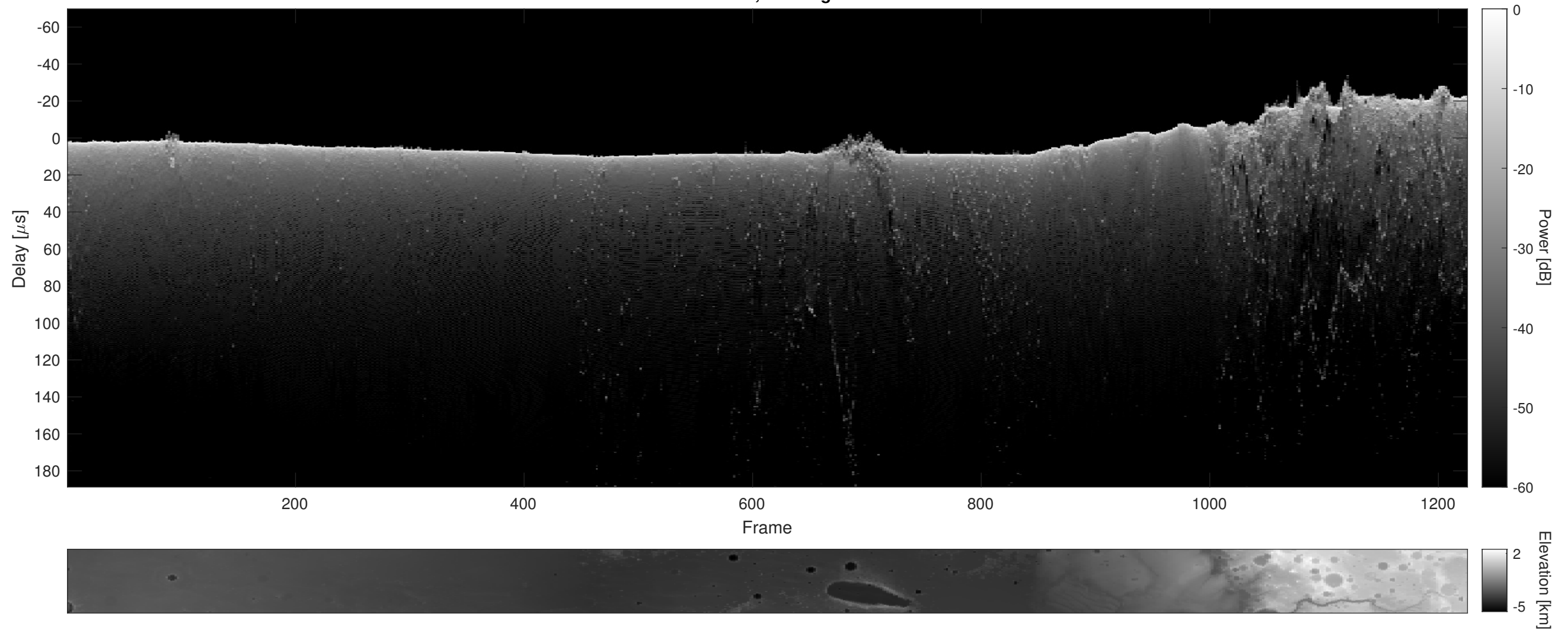
Orbit 5233, Cluttergram
