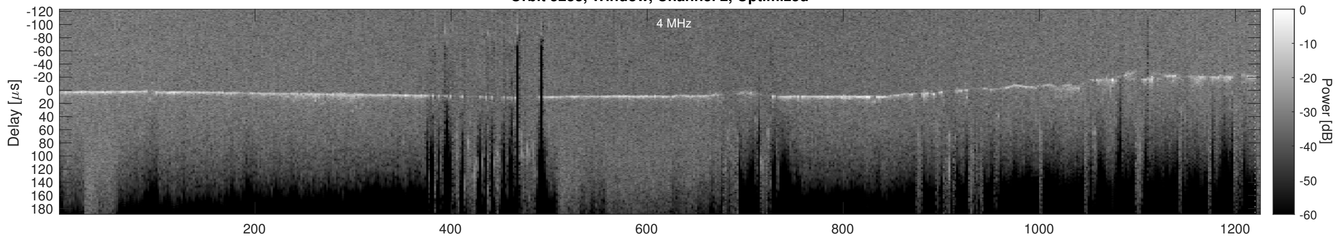
Orbit 5233, Cluttergram
