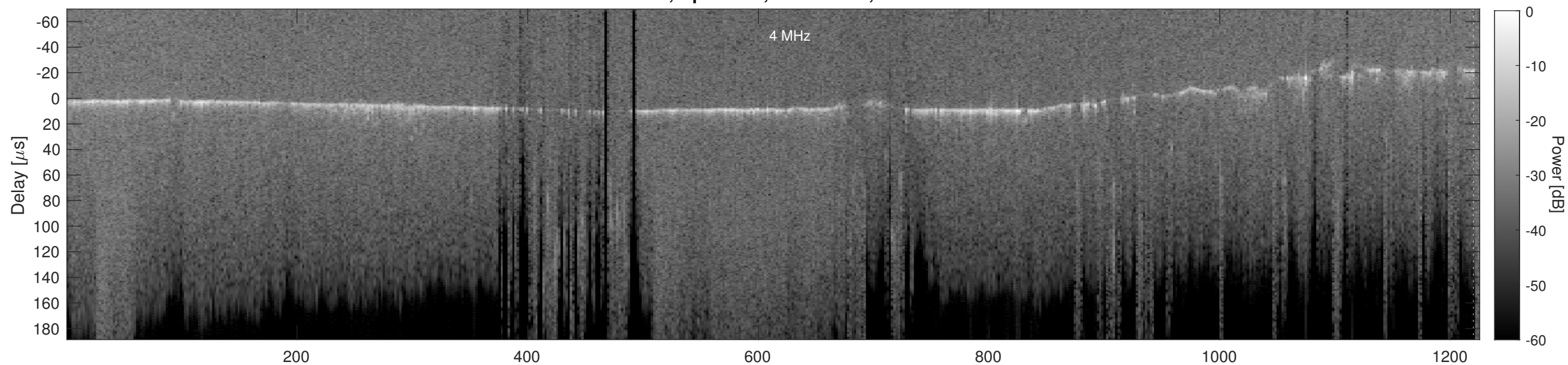
Orbit 5233, Cluttergram
