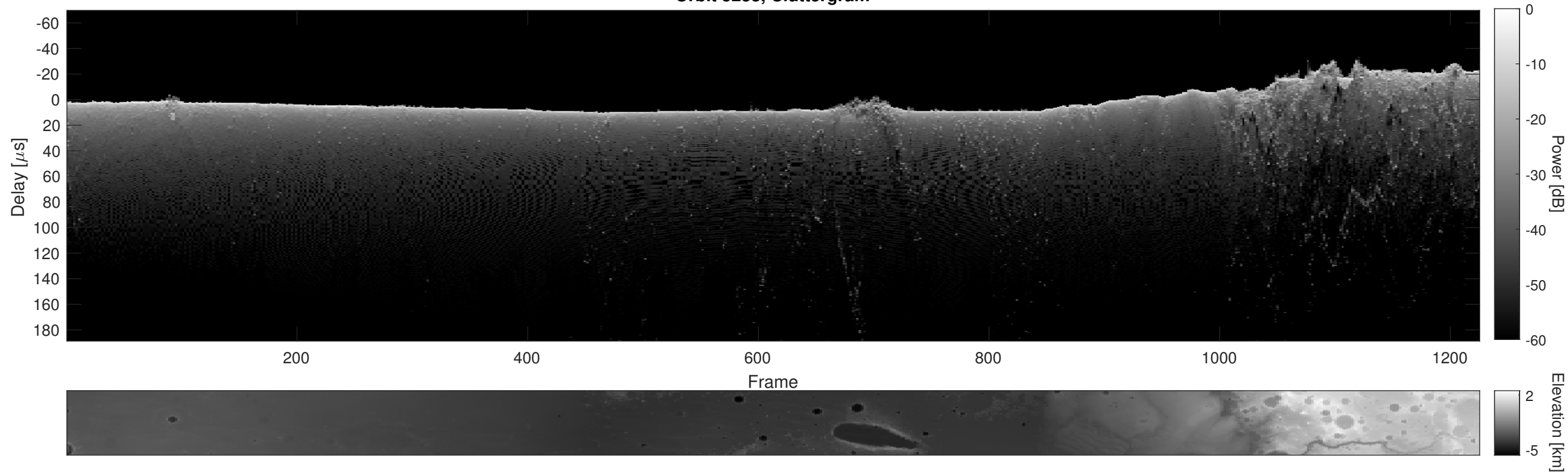
Orbit 5233, Cluttergram
