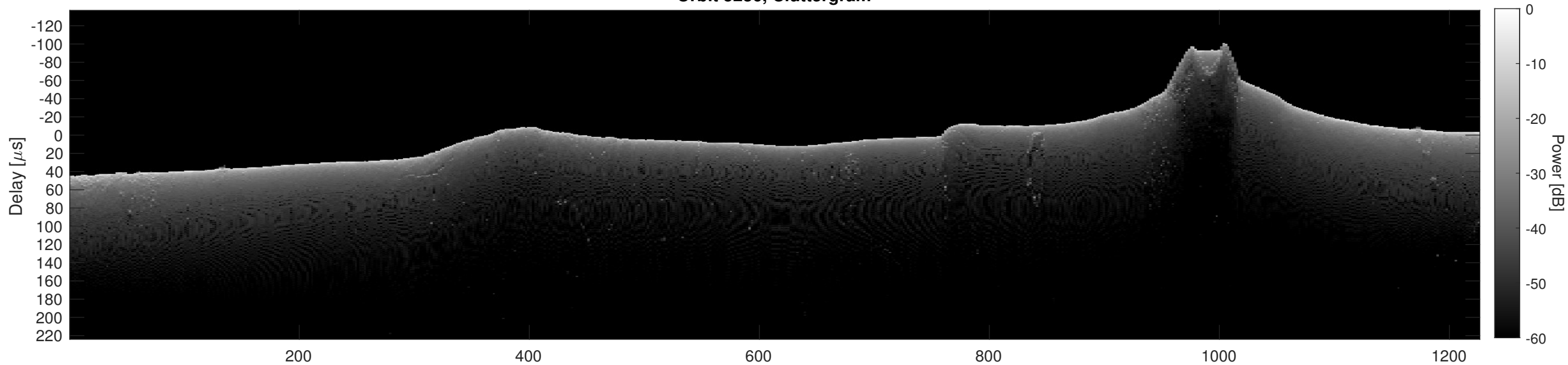
Orbit 5236, Cluttergram
