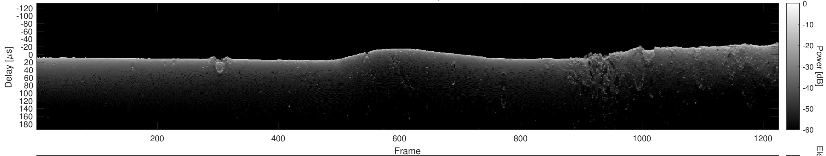
Orbit 5237, Cluttergram
