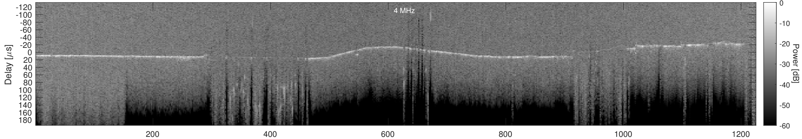
Orbit 5237, Cluttergram
