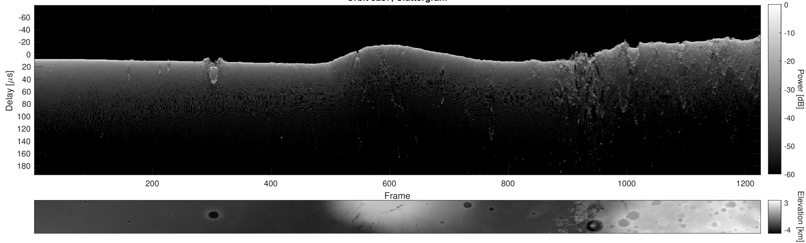
Orbit 5237, Cluttergram
