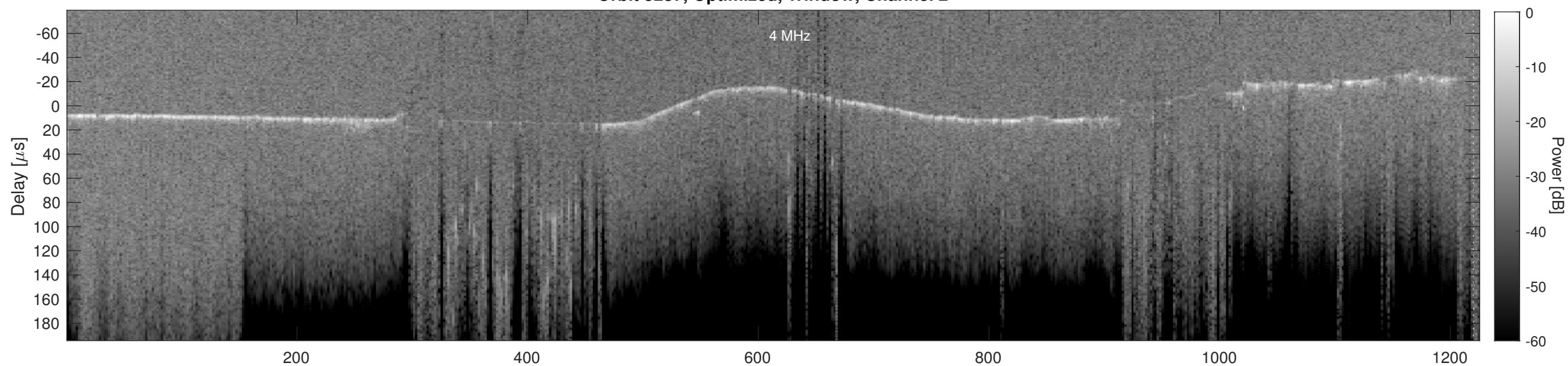
Orbit 5237, Cluttergram
