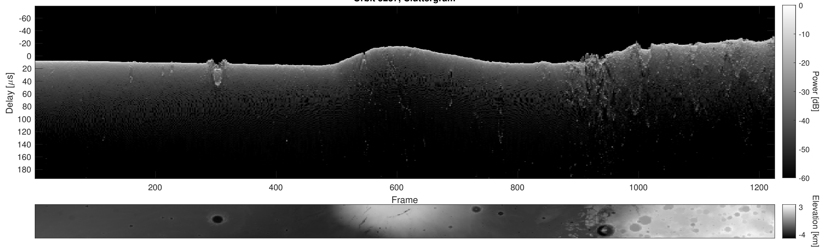
Orbit 5237, Cluttergram
