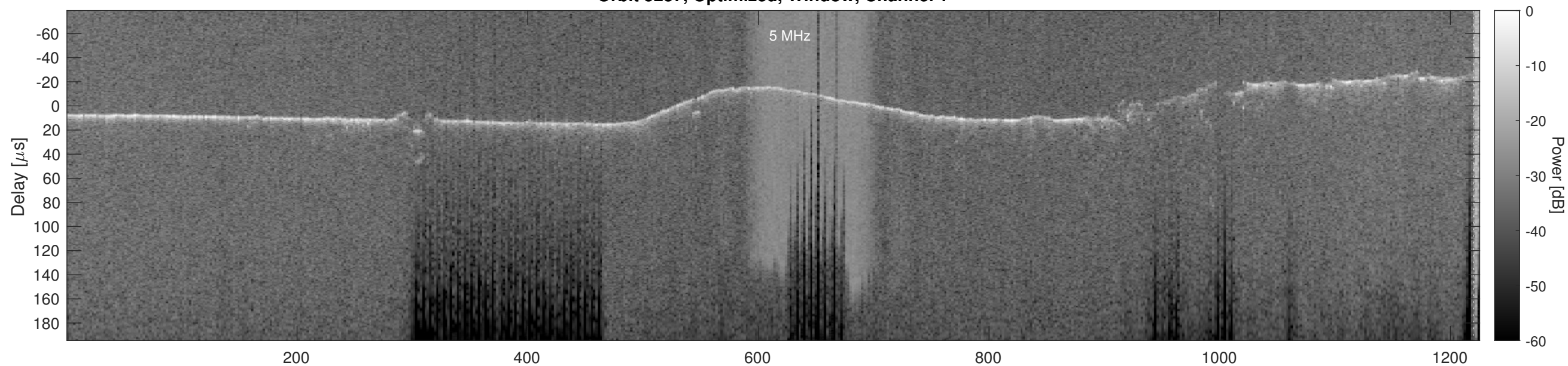
Orbit 5237, Optimized, Window, Channel 2
