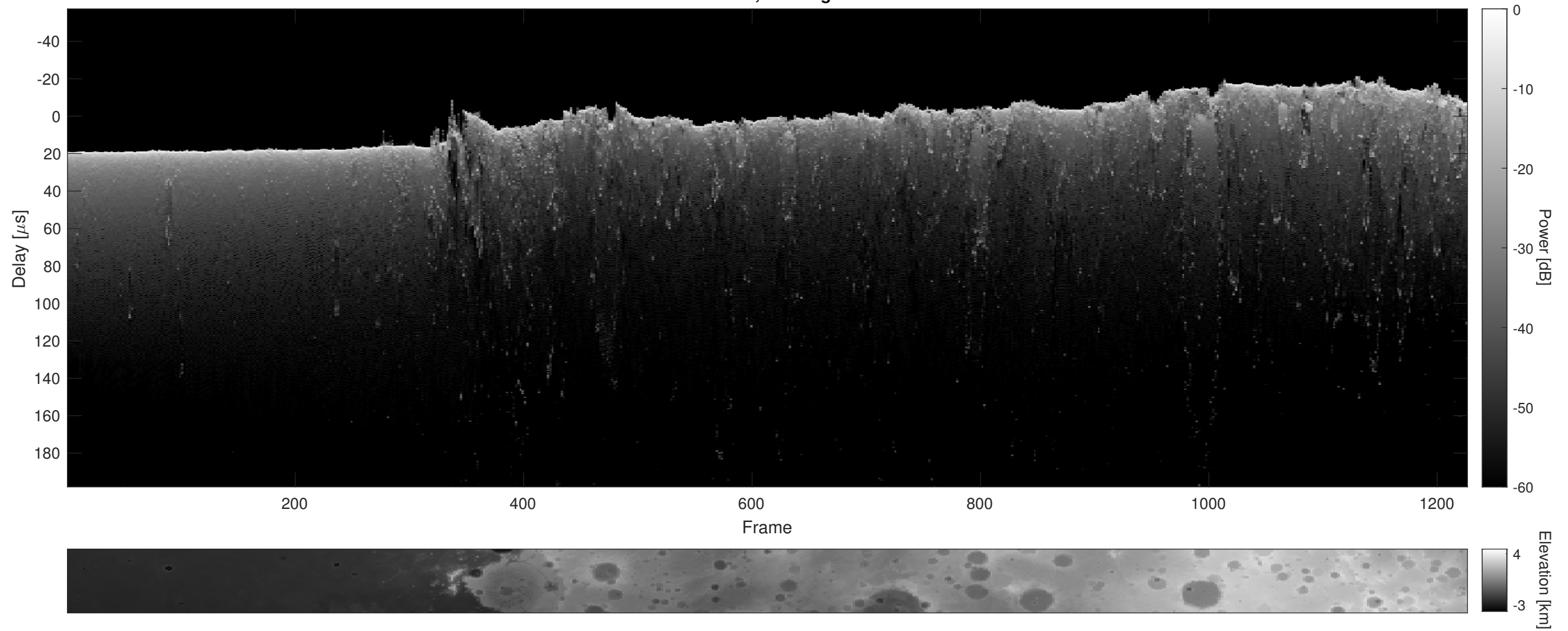
Orbit 5238, Cluttergram
