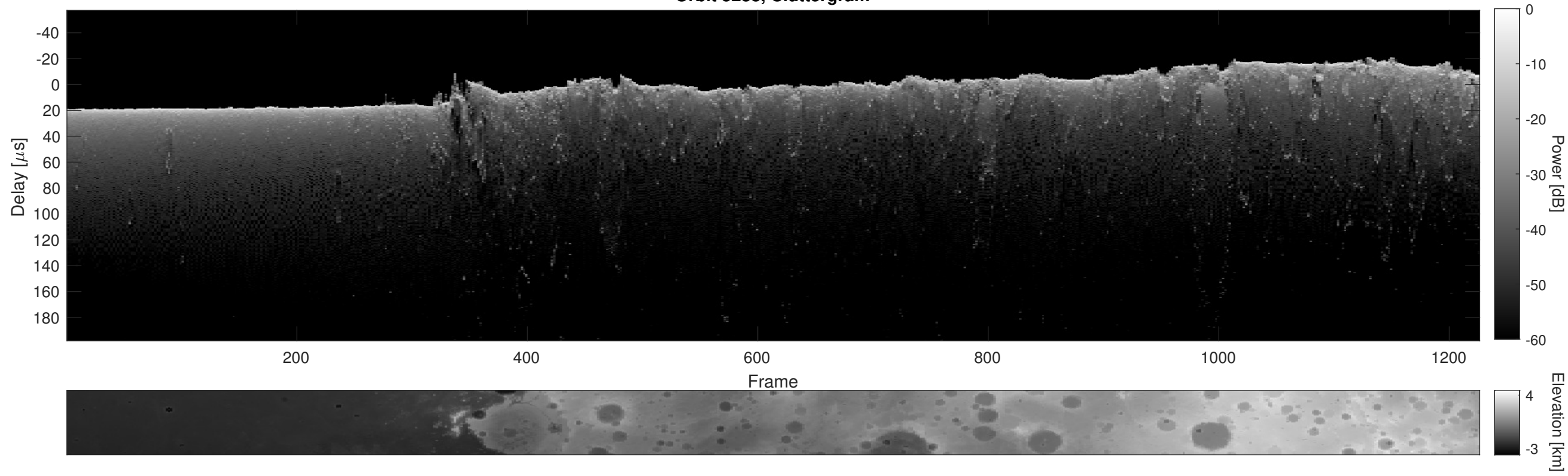
Orbit 5238, Cluttergram
