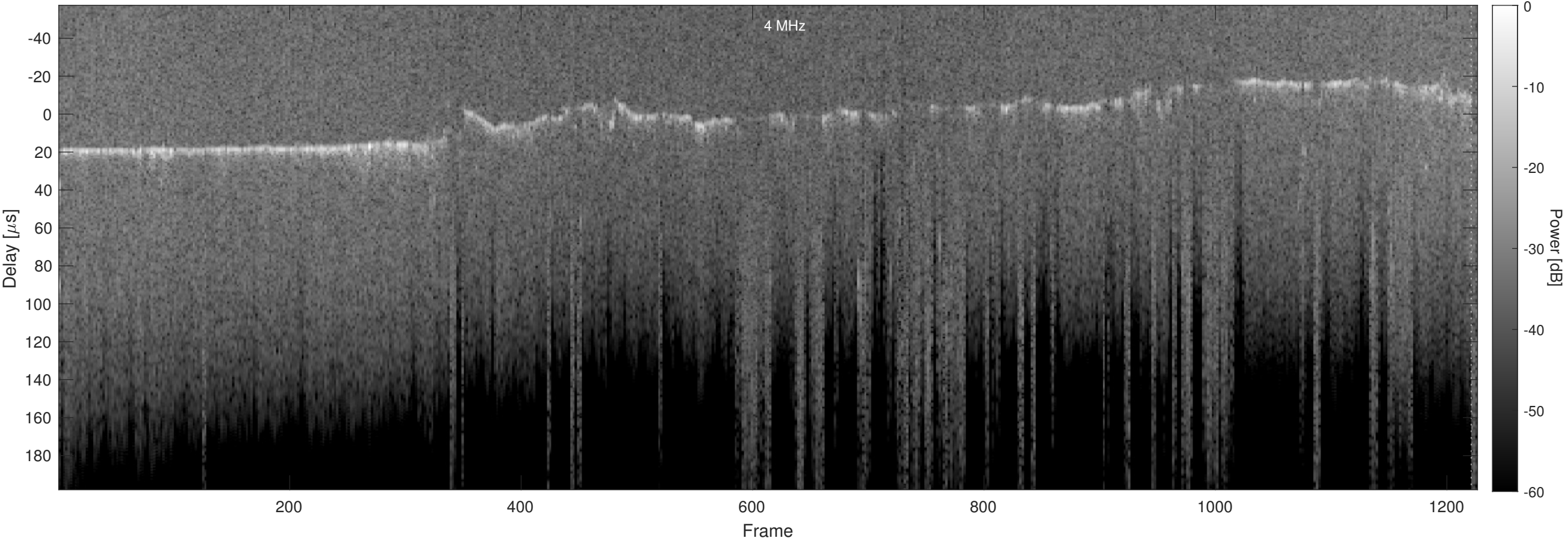
Orbit 5238, Optimized, Window, Channel 2
