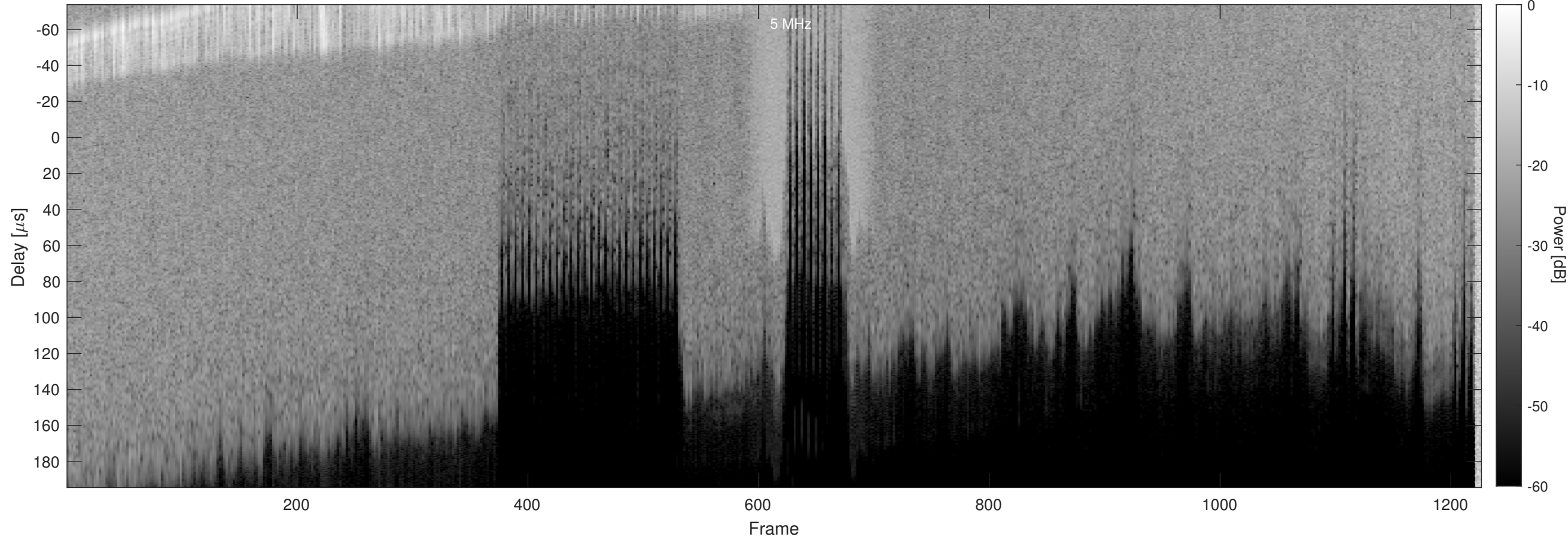
Orbit 5241, Chapman, No Window, Channel 2
