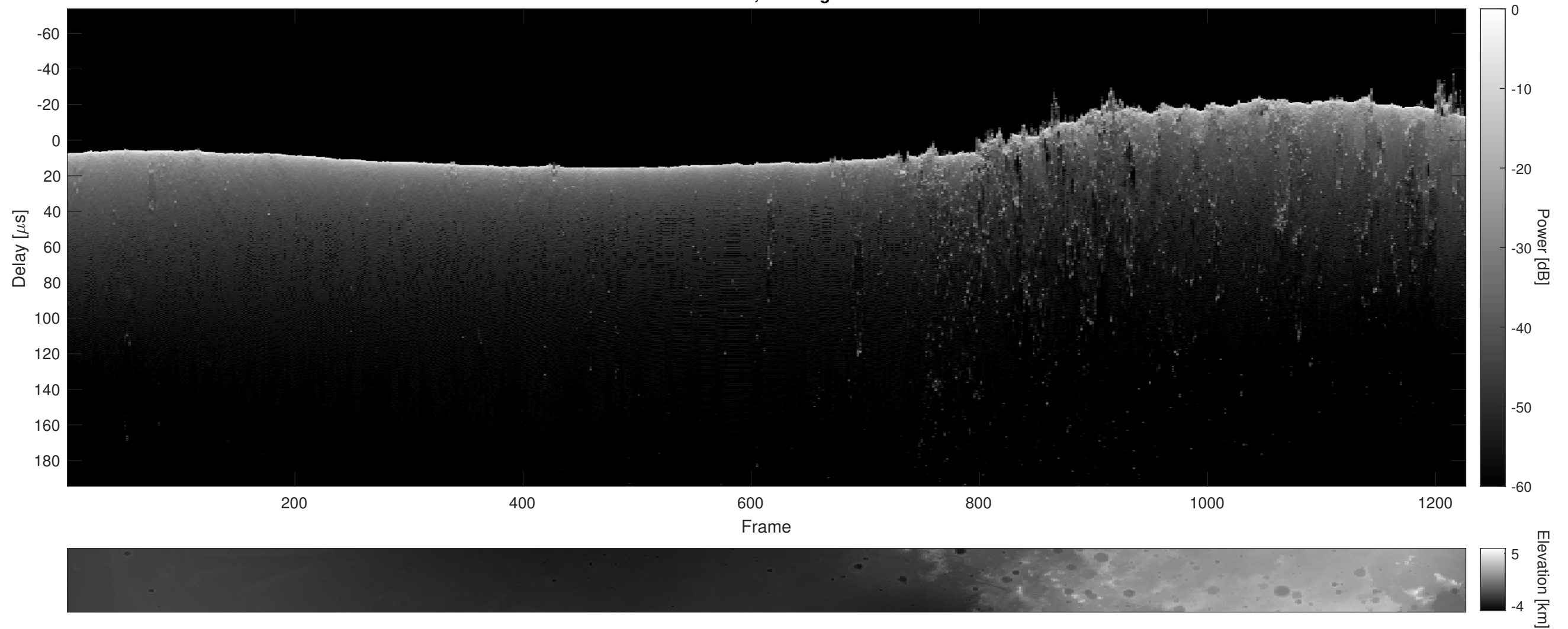
Orbit 5241, Cluttergram
