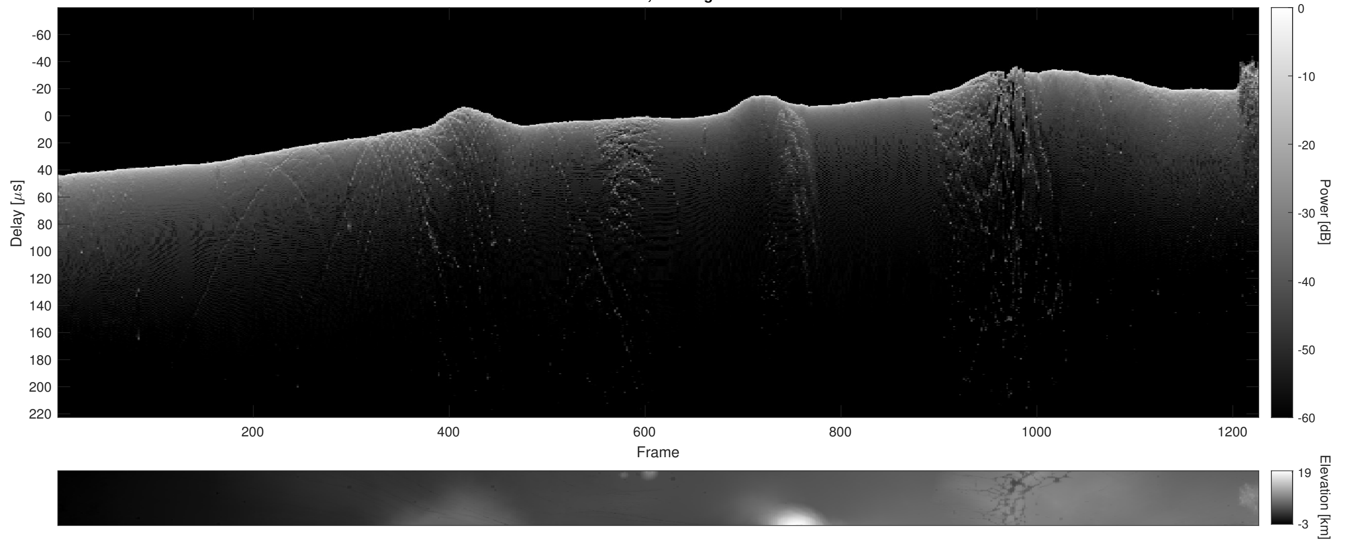
Orbit 5243, Cluttergram
