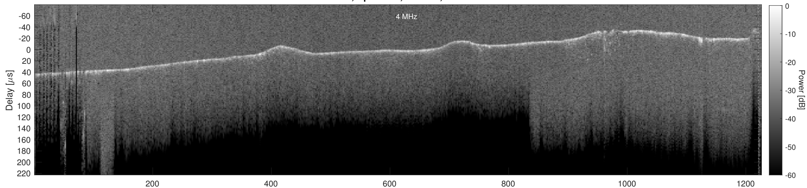
Orbit 5243, Cluttergram
