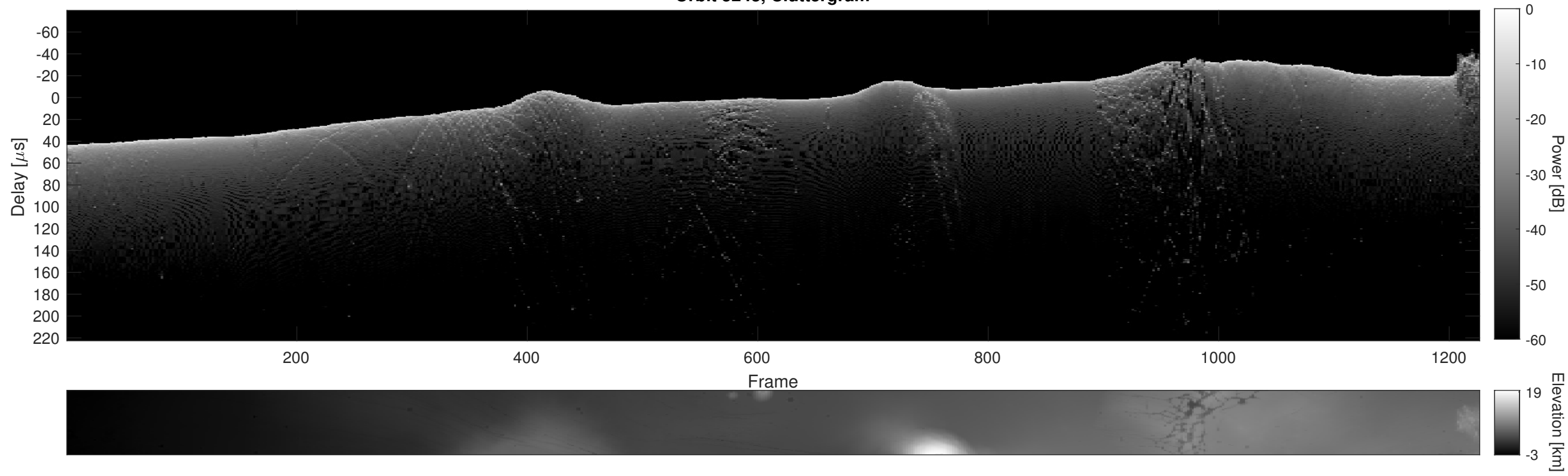
Orbit 5243, Cluttergram
